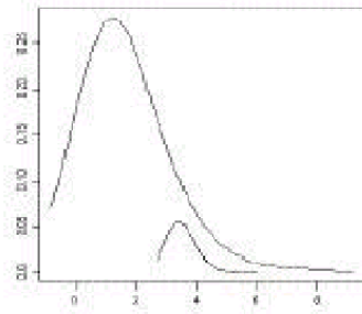
Driven system: skewed subclade
