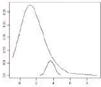
Passive system: symmetric subclade
